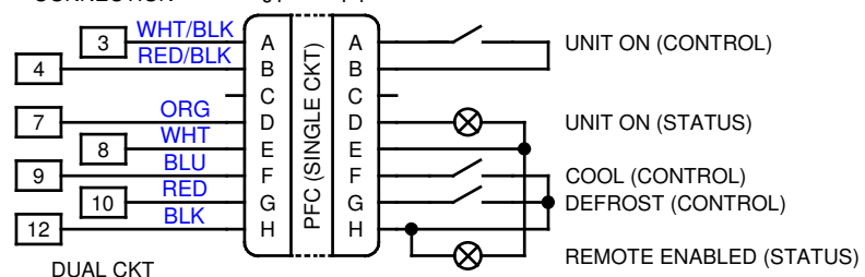
DUAL CKT REMOTE CONTROL CONNECTION
