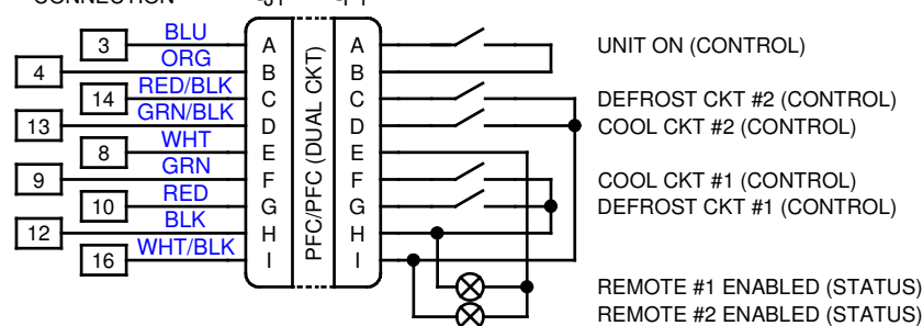
DUAL CKT REMOTE CONTROL CONNECTION
